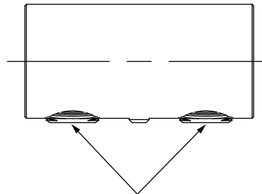
3/8" - 24 Set Screws (2 Places)
